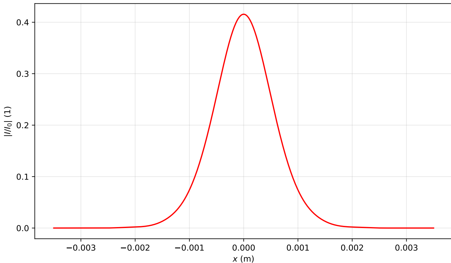
Intensity profile I(x, y = 0, z = 3.821)/I_0 , P_{in}=0.5P_{cr} , artificial time
